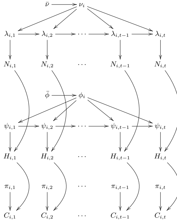
Fig 3: Graphical model of the continuum-level homeless population. In metro i in year t , the total population is modeled by N_{i,t} , the homeless population is modeled by H_{i,t} , and the number of homeless counted is modeled by C_{i,t} . The dynamical processes and associated parameters are outlined in Sections 3.1 - 3.3.
