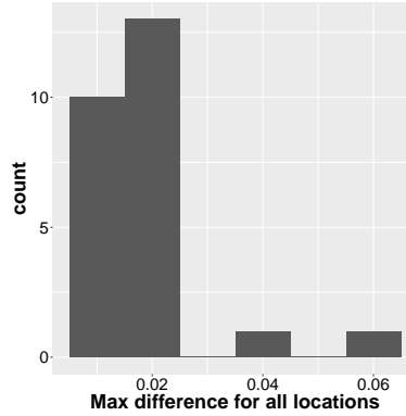
Fig 7: The maximum difference in posterior means of \phi_1, \dots, \phi_{25} for 10 different MCMC simulations. Each of the 25 points in the histogram corresponds to \max_j |\phi_i^{(j)} - \phi_i^{(1)}| , for each of the 25 metros denoted by i . The superscript index j denotes the MCMC simulation. The very small differences indicate that our MCMC simulations generate reproducible inference in \phi_i .
